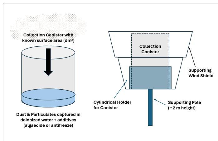
Fig 2. Components of a Dustfall Sampler
